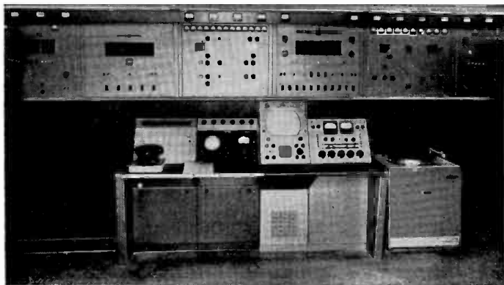
Main room of the WTVJ transmitter building showing visual and aural exciters, and amplifiers and control console.
